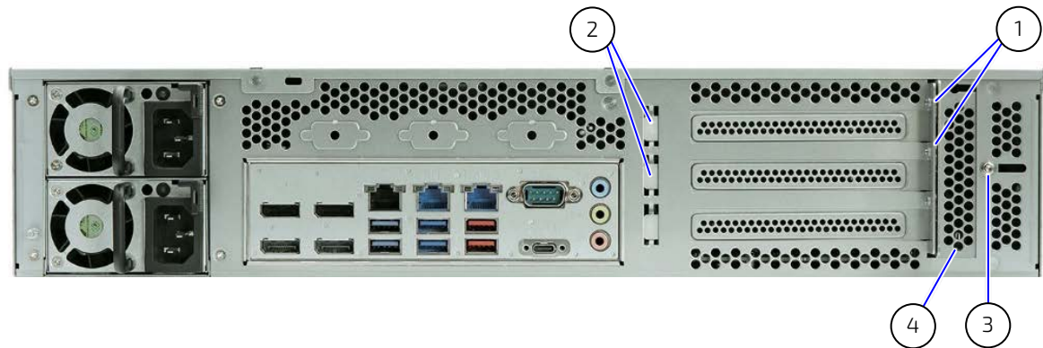
Figure 20: Installing Riser Card Expansion Cards
