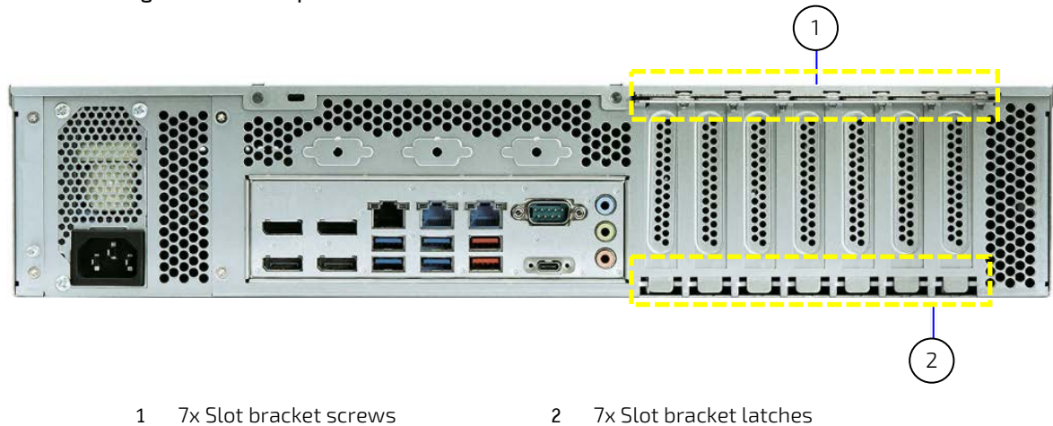
Figure 19: Installing Low Profile Expansion Cards
