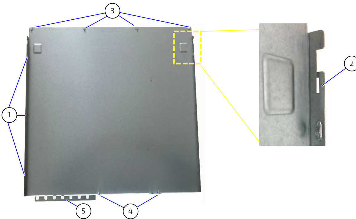
Figure 16: Cover Underside (low profile)
