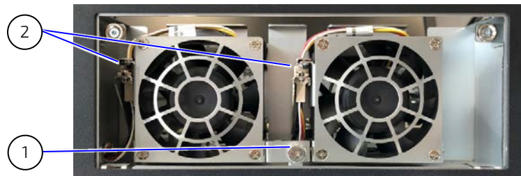
Figure 29: Removing a System Fan
