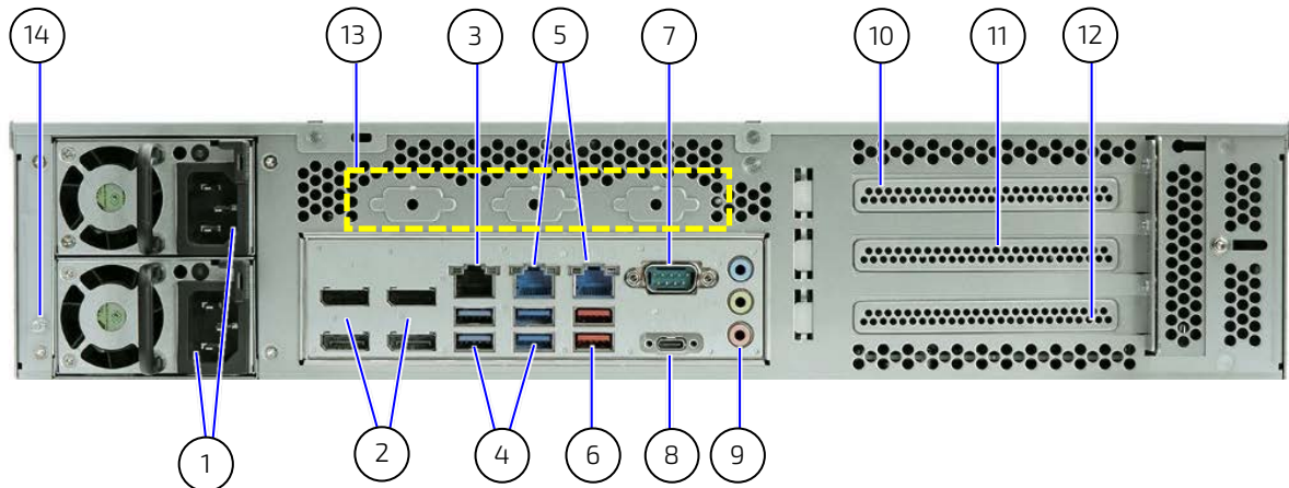
Figure 10: Rear Panel (riser card)
